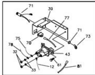
DETAIL OF ELECTRIC STARTER SWITCH
