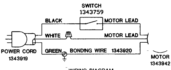
WIRING DIAGRAM
