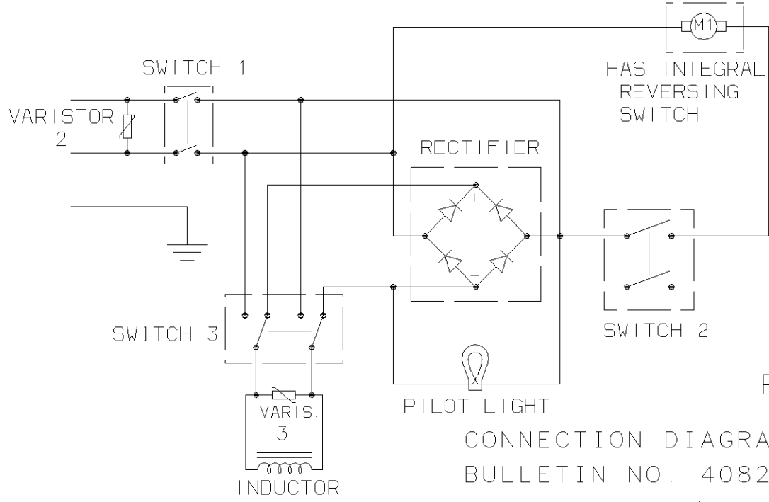
SCHEMATIC DIAGRAM
