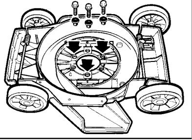
MOTOR MOUNT (Bottom View): Items 53, 54 assembled in 3 locations indicated.
