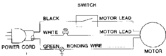
WIRING DIAGRAM
