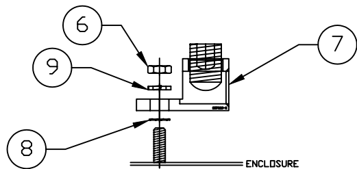
DETAIL A-A (GROUND LUG ASSEMBLY)
