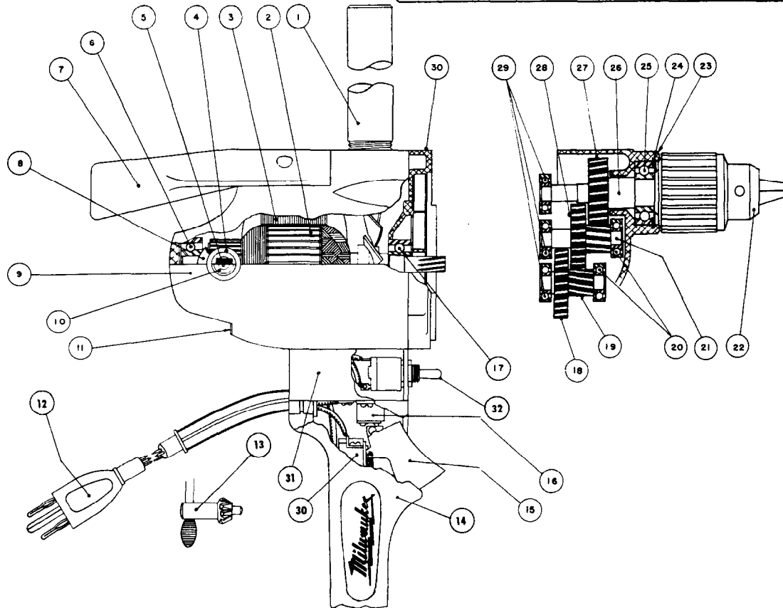
ILLUSTRATED PARTS
