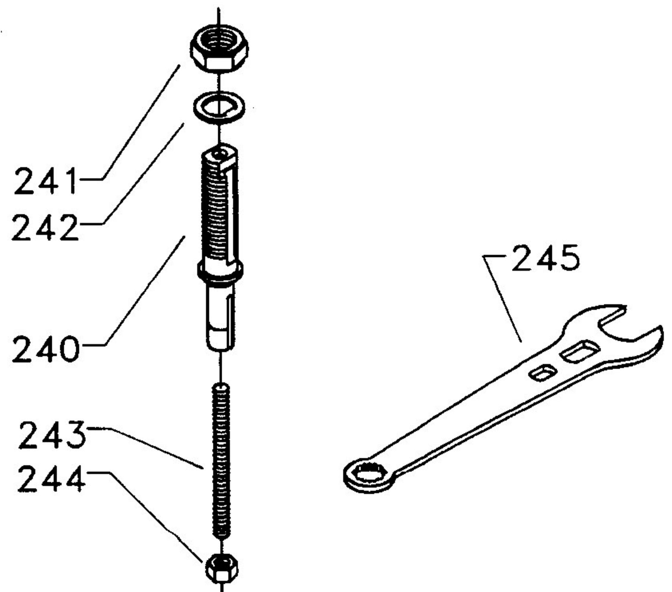
43-143 3/4" SPINDLE ASSEMBLY
