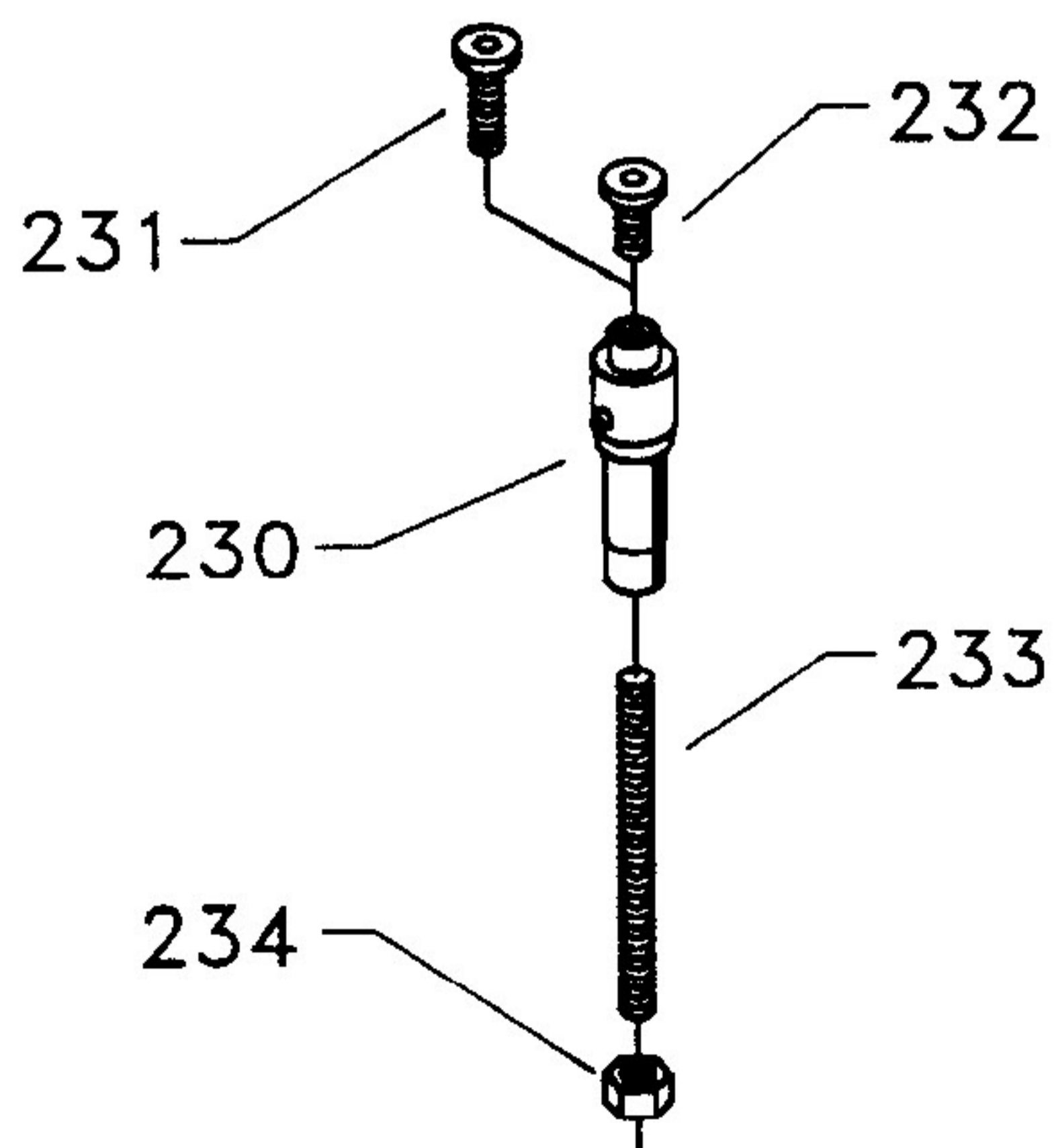
43-144 STUB SPINDLE
