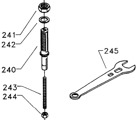
43-143 3/4" SPINDLE ASSEMBLY
