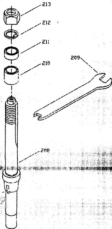
43-808 1" SPINDLE
