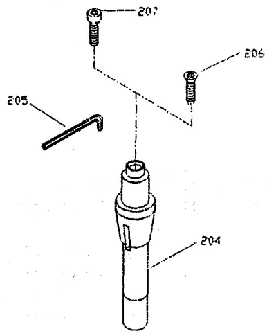
43-809 STUB SPINDLE
