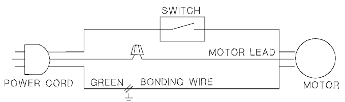
WIRING DIAGRAM
